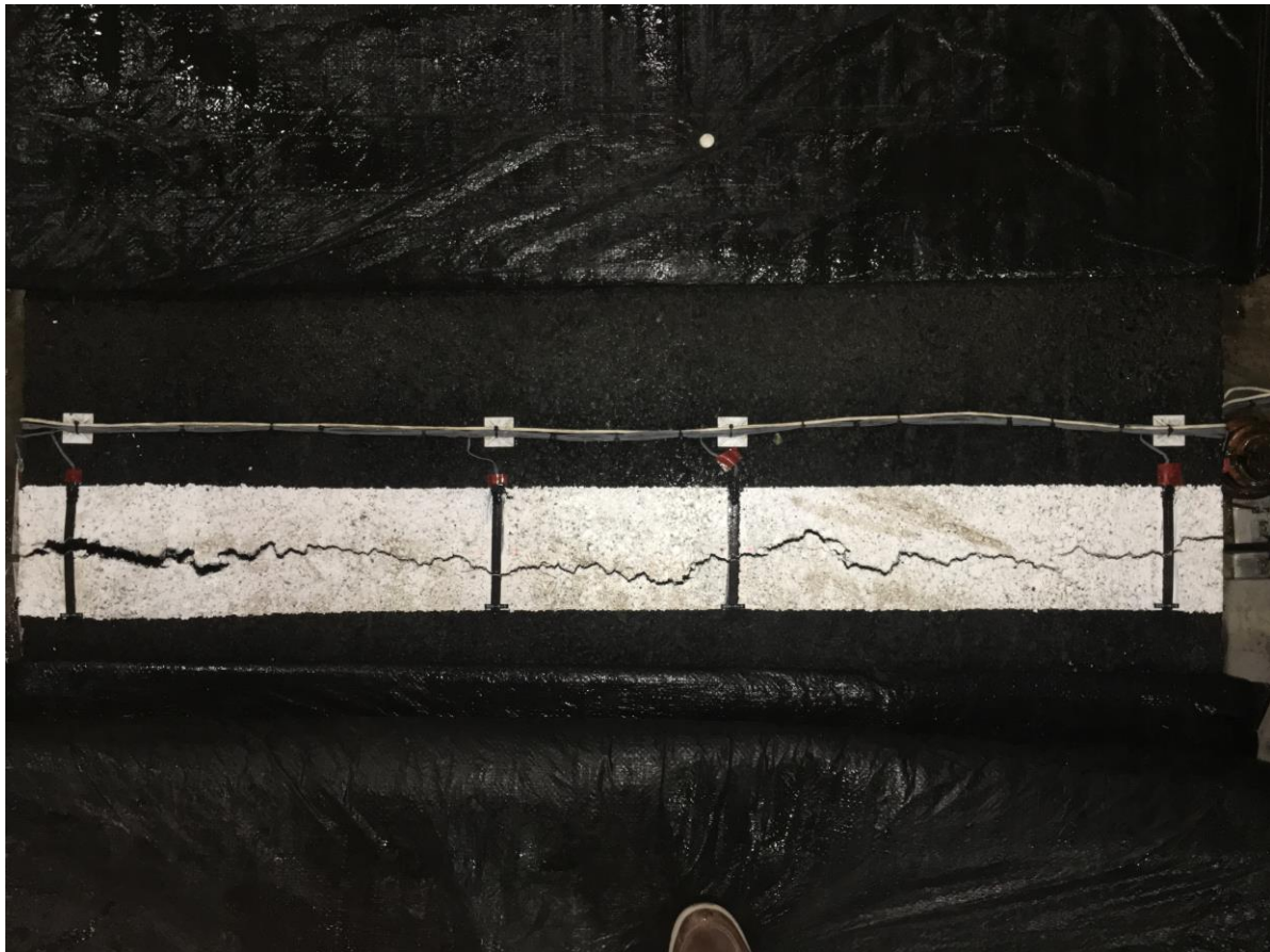
Fig 8 North Section Surface Crack
